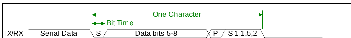
Figure 18-1 UART Serial Data Format
