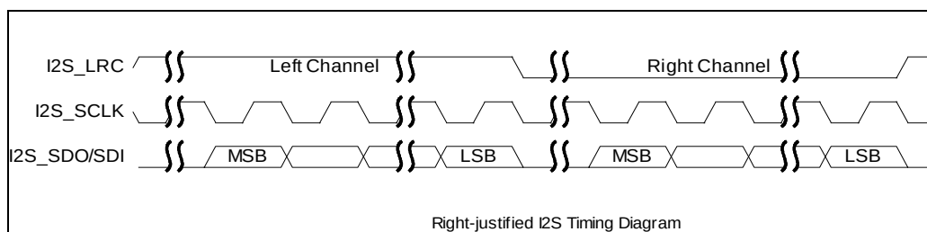
Figure 22-4 I2S Right-justified Timing Diagram
