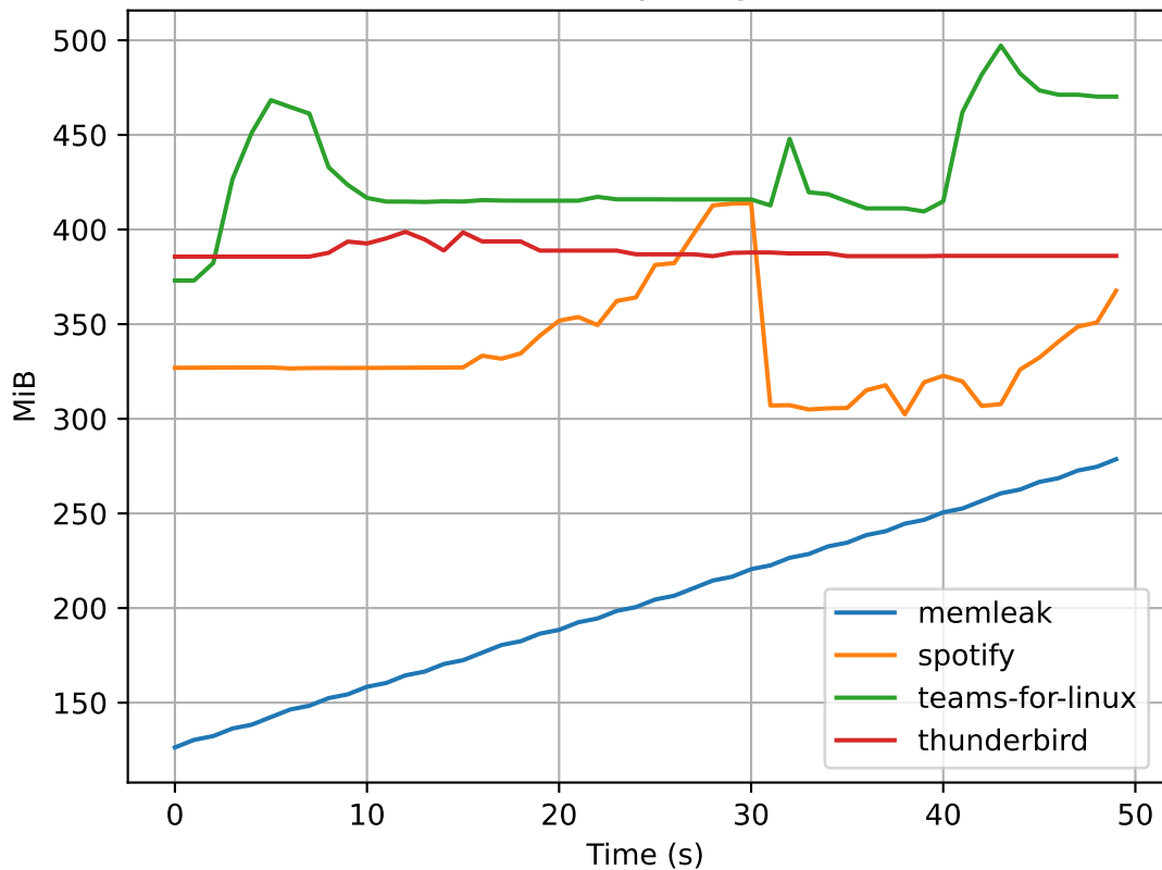
Memory usage
